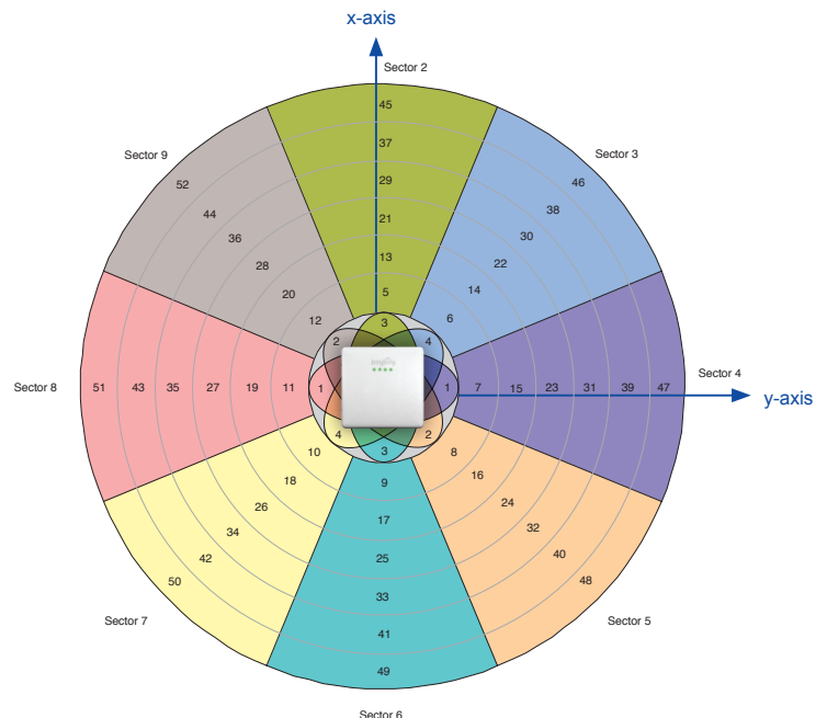
The Speedway xArray reader system can distinguish 52 different antenna beams providing location assignment and wide-area monitoring.
